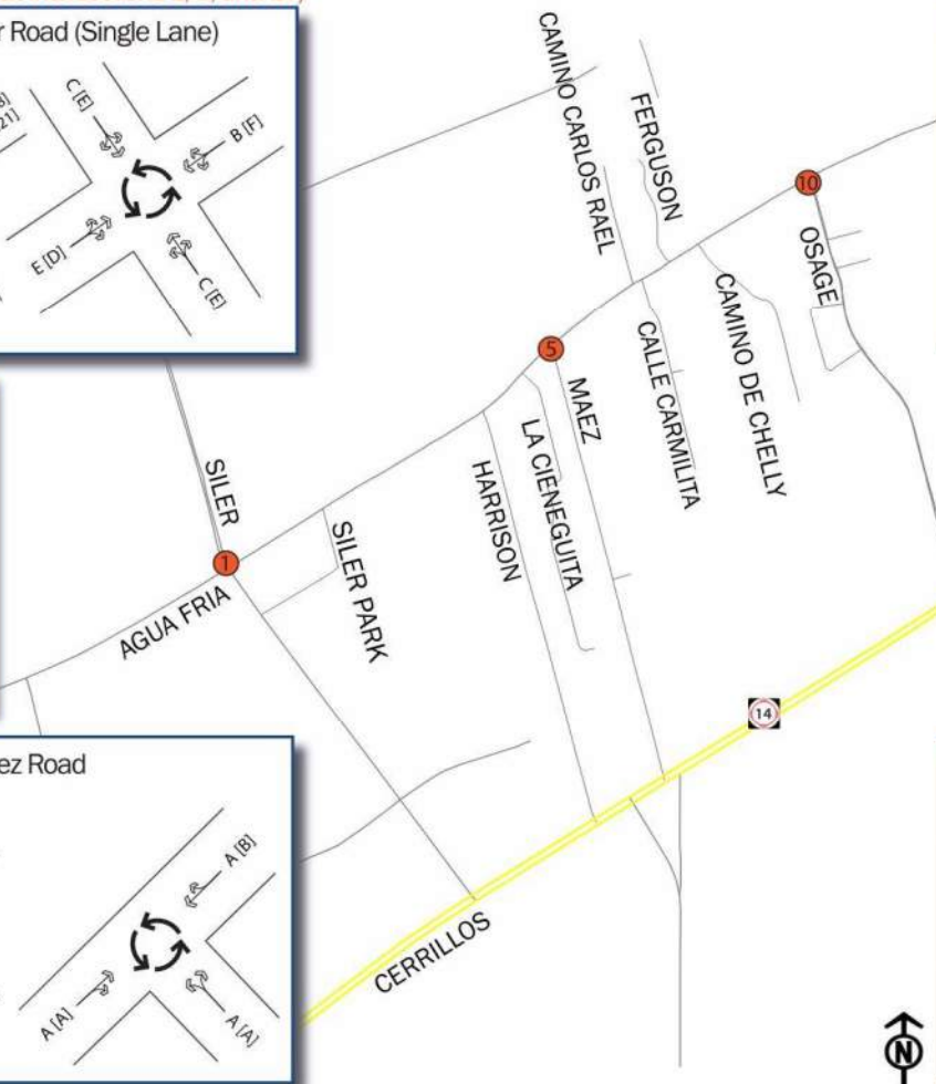
Figure 55: Roundabout Traffic Volumes – Friday
