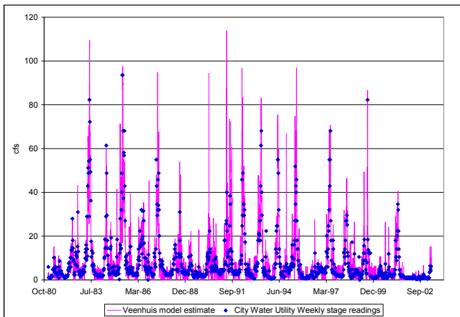
Figure A-1. Modeled on the Santa Fe River at the above McClure Reservoir gage and inflow based on weekly readings of flume levels 1981 to 2002.
