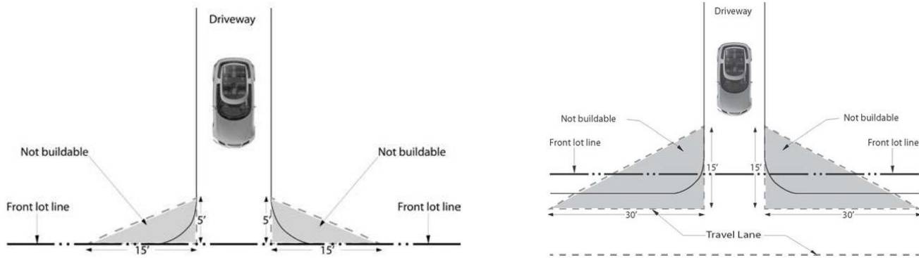
Illustration 14-7.1-1 Visibility at Driveways on Lanes and Sub collectors
