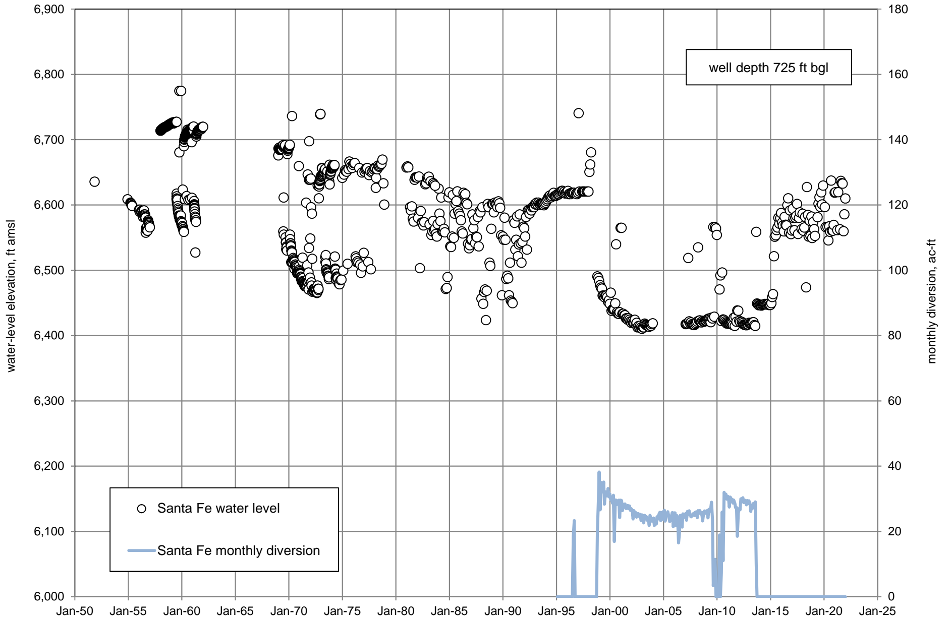
Figure B6. Water-level elevations for Group B Santa Fe Well, Northwest Well Monitoring Plan, Santa Fe, New Mexico.
