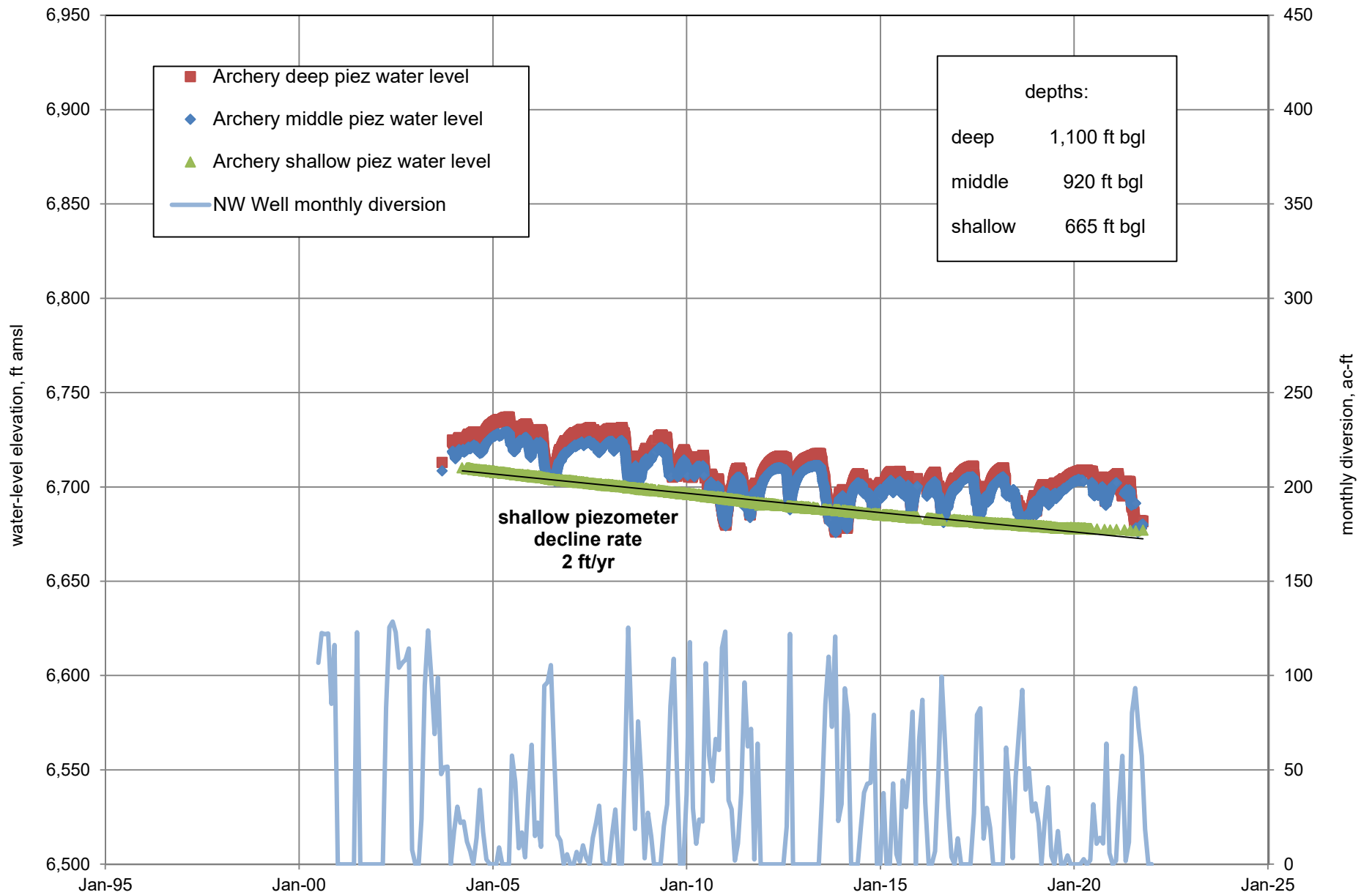
Figure D1. Water-level elevations for Section 6.b wells Archery shallow, middle, and deep piezometers, Northwest Well Monitoring Plan, Santa Fe, New Mexico.
