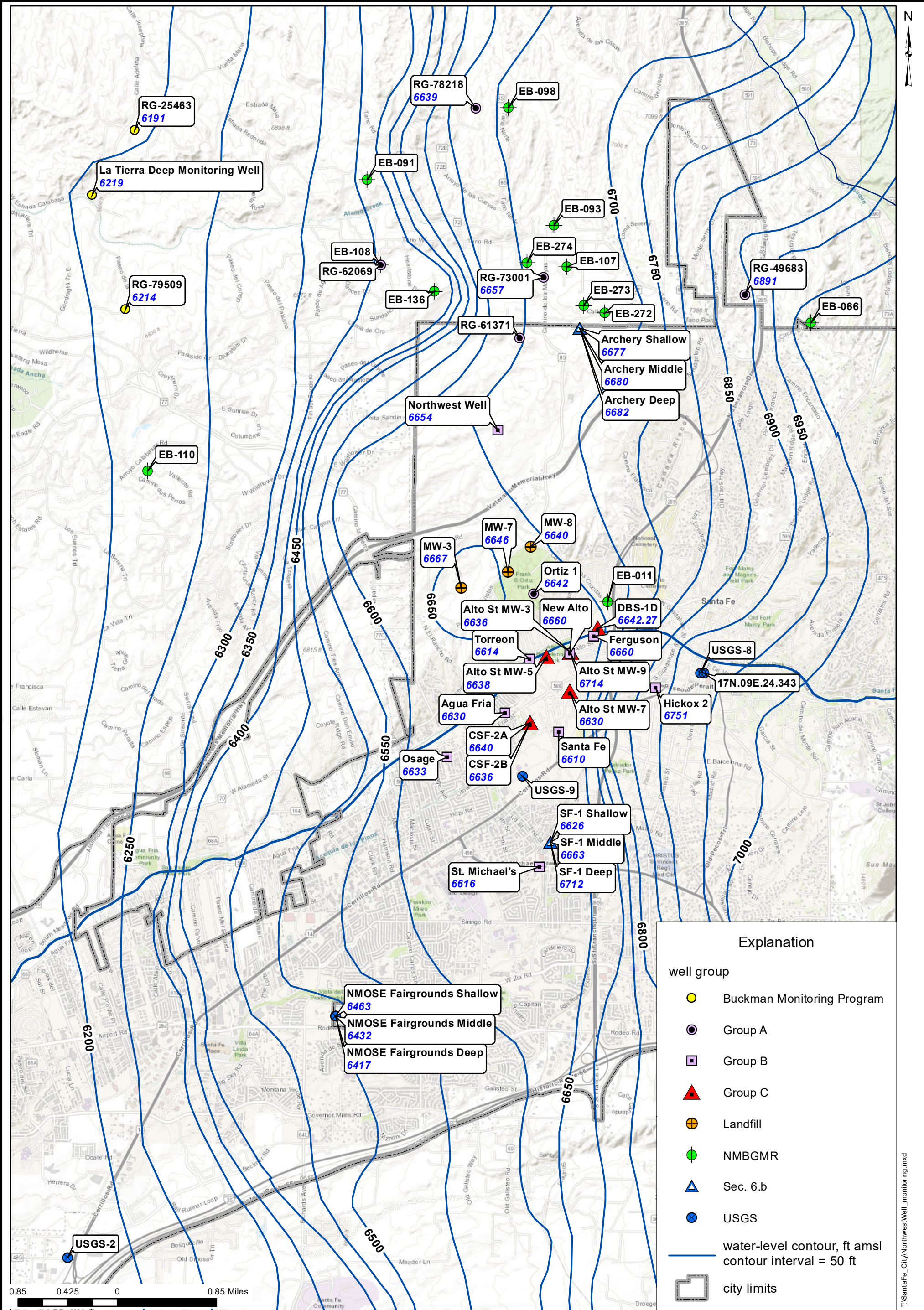
Figure 3. Map showing water-level elevation contours for Northwest Well and City Well Field area representing current conditions, Santa Fe, New Mexico.
