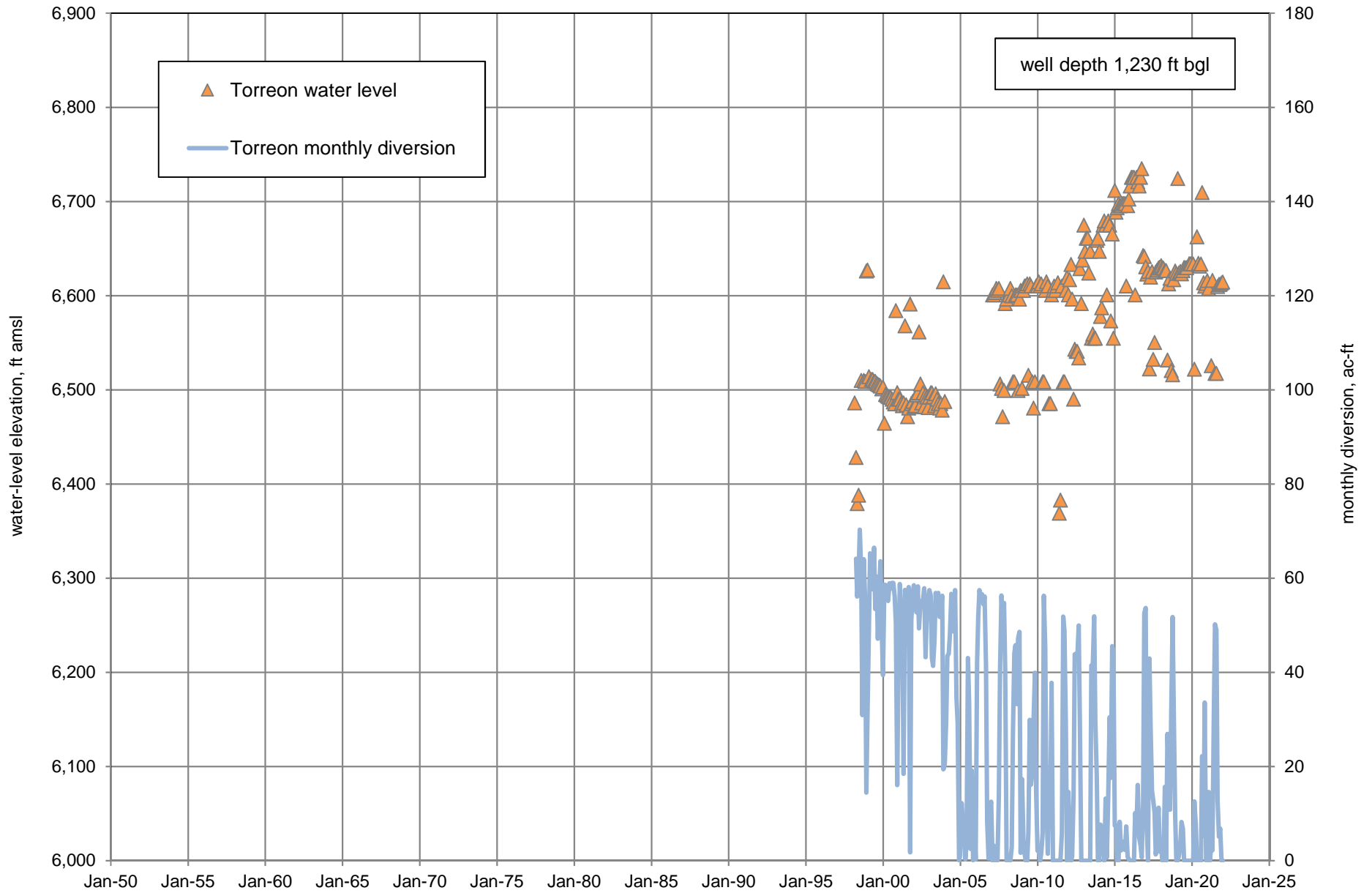
Figure B8. Water-level elevations for Group B Torreon Well, Northwest Well Monitoring Plan, Santa Fe, New Mexico.
