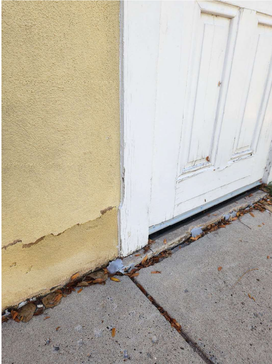
Example of deterioration and apparent settlement of wall and stucco.
